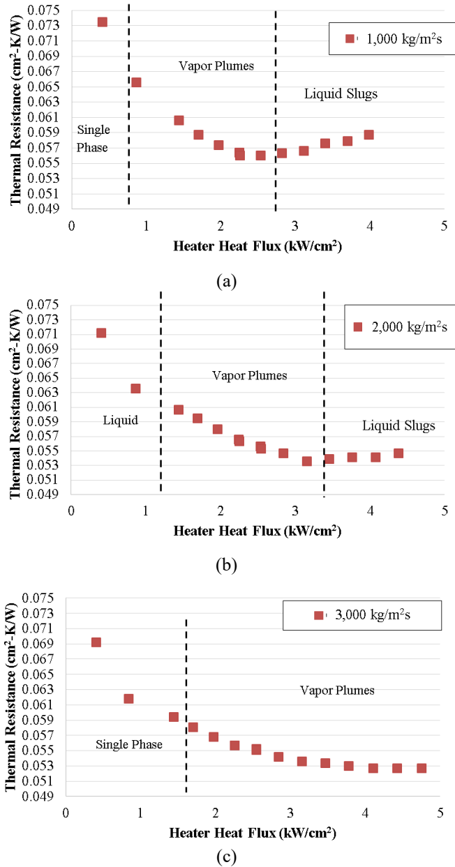
Fig. 12 Thermal Resistance vs heat flux for Gen 3 device: (a) G=1000 \text{ kg/m}^2\text{s} (b) G=2000 \text{ kg/m}^2\text{s} (c) G=3000 \text{ kg/m}^2\text{s} , mapped into flow regimes described in Fig. 13.
